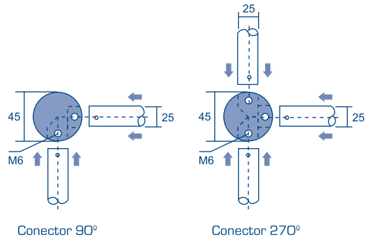
Conector 90°
